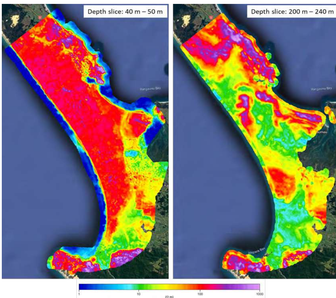
Figure 4. Mean resistivity maps with depth slices of 40 m to 50 m, and 200 m to 240 m.
