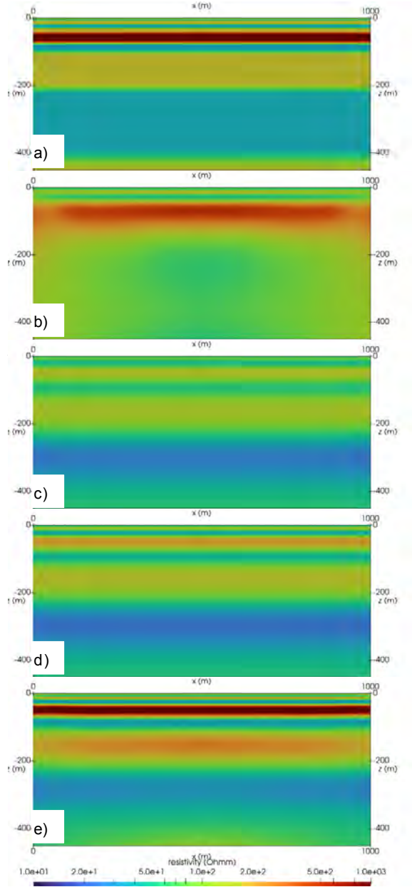
Figure 4. Synthetic model and inversion results. a) resistivity section of a MPA IP simulation of electrical properties; b) inversion model of DCIP data; c) inversion model of AEM+ground EM data; d) inversion model of AEM+ground EM+tTEM data; e) joint inversion of all inductive and galvanic data.
