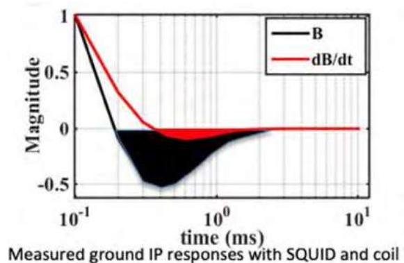
Figure 1: Comparison over polarizable ground of measured decays between coil and SQUID sensors using the same transmitter and receiver locations.
