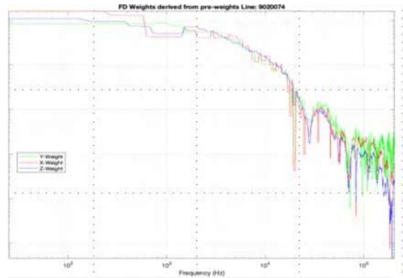
Figure 6 : Tikhonov Regularisation used during Deconvolution of TEMPEST System Response
