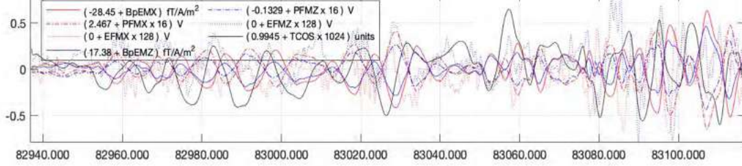
NOISE MONITORS: Spherics - SPH, Powerline - PWLF, Base Frequency - LOWF, Figure 3: The X and Z components of the windowed, 100% duty-cycle Bfield obtained from processing a high-altitude reference line as if it was a survey line. This represents the noise during straight and level flight, and its variance may be used as noise estimate when working with windowed data.
