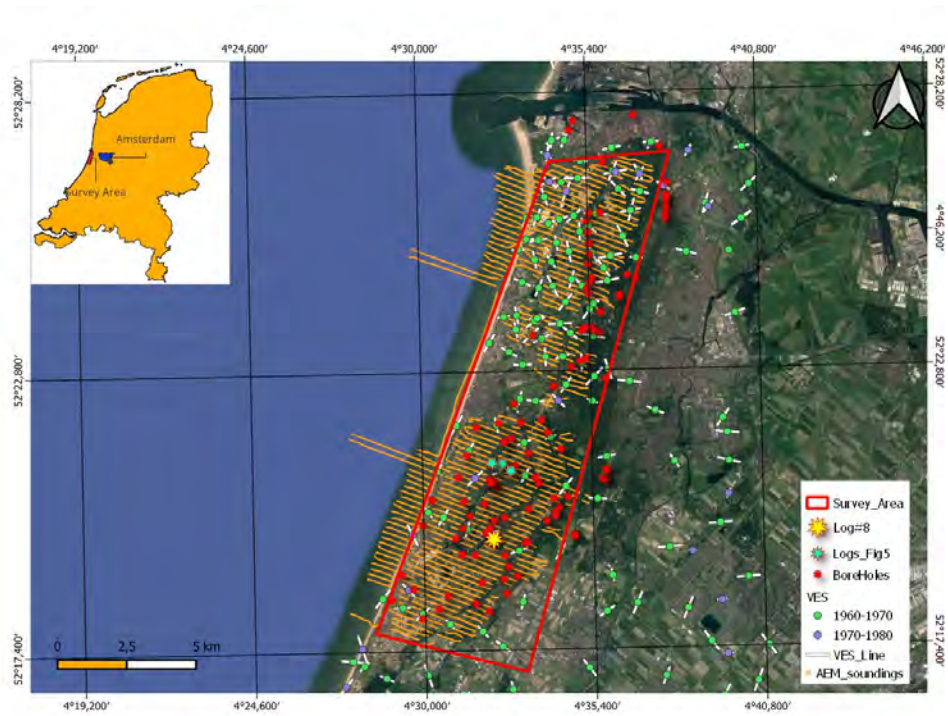
Figure 3. Survey area and sounding locations: red polygon – inversion area; orange dots – AEM soundings; red stars – borehole resistivity logs; yellow and green stars – logs presented in Fig. 5 and Fig. 6; green dots – VES soundings from the ‘60s; purple dots – VES soundings from the ‘70s; white bars: VES orientations.
