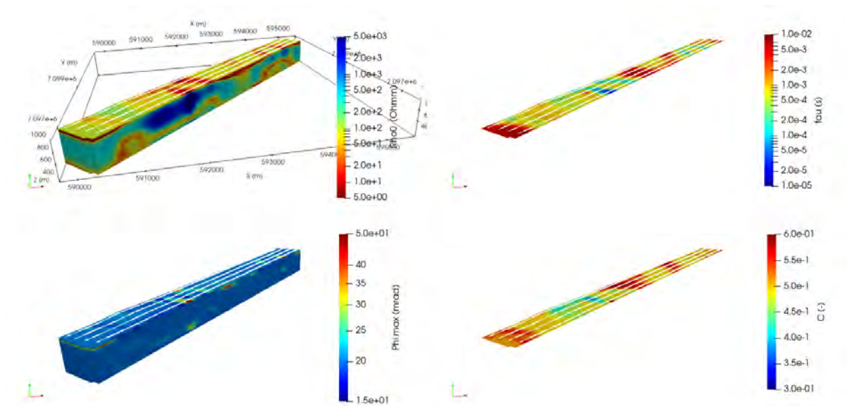
Figure 5. EEMverter inversion model of the Valen VTEM survey. Top left – resistivity model; Bottom left – chargeability (maximum phase) model; Top right – model of the time constant \tau ; Bottom right – model of the spectral exponent C . White lines represent the acquisition lines.
