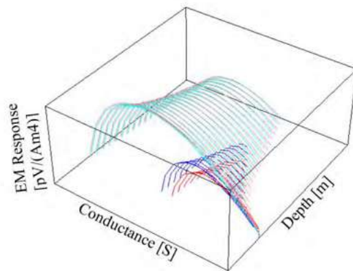
Figure 3: A 3D conductance-depth nomogram. The conductance varies from 0.1 to 106 S (log scale), depth varies from 20 to 500 m (linear scale) and EM response varies from 0-380 \text{pV}/(\text{Am}^4) (log scale). The cyan and blue traces are the first and last channels of 25 Hz data, while the light red (very close to cyan traces) and dark red traces are the first and last channels from 12.5 Hz modelled data.
