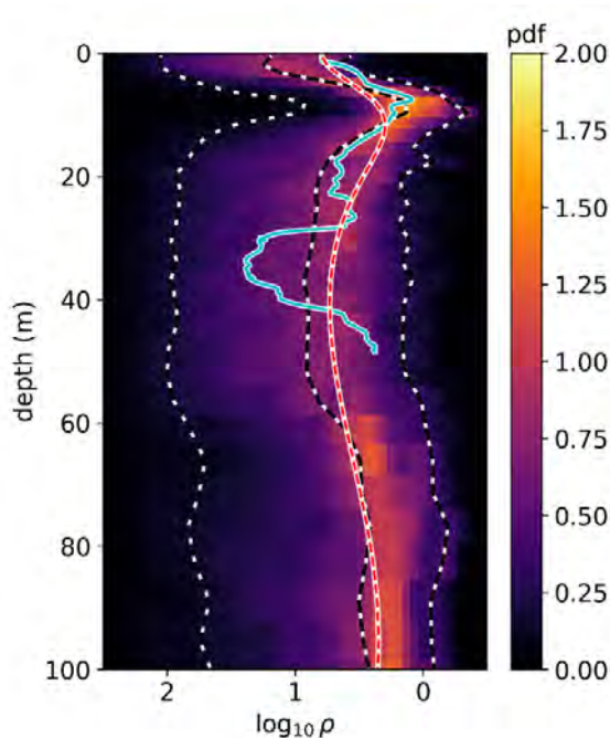
Figure 1. Deterministic and probabilistic inversion of AEM data at a sounding close to a logged borehole. Induction log values are shown with a blue line, and deterministic inversion results taking geometry nuisances into account are shown with a dashed red and white line. Higher probability resistivities are shown with hotter shades, and
