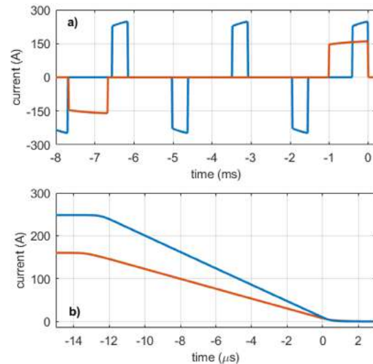
Figure 5. a) Plot of the current waveform transmitted in the 2021 survey in Norway (orange) together with the current waveform transmitted in the 2023 survey in Denmark (blue). b) Zoomed-in view of the current turn-off shape and duration for the waveforms in panel a. Notice the change in time units between the two panels.
