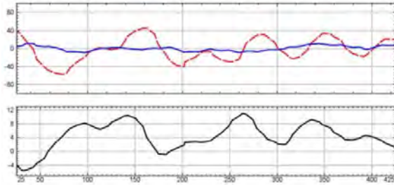
Figure 1. In the absence of the secondary field: measured (red) and corrected (blue) values in ppm as a function of time in samples ( \sim 10 Hz) for one of the EQUATOR's harmonics (230 Hz). The bottom chart is the receiver axis inclination in degrees.
