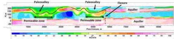
Figure 3. Spatially-constrained inversion of the conducted data with interpretation.
