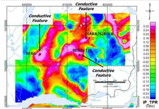
B) ZTEM TOTAL DIVERGENCE (DT) IN-PHASE (90 Hz)
