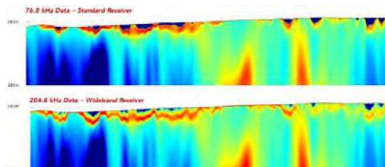
Figure 2: Conductivity Depth Images comparing two data sets that have been sampled at different acquisition rates; 76.8kHz and 204.8kHz.
