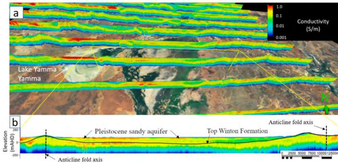
Figure 2. a) Oblique view of of AEM conductivity sections across the central Cooper Creek floodplain east of Lake Yamma Yamma, overlain on true colour visible satellite imagery. b) AEM section 1014001 showing both the flat-lying, conductive Pleistocene sandy aquifer sediments and the gently folded Winton Formation. The floodplain, which contains up to 150 m of Cenozoic sediment, lies within a broad syncline between two anticlinal folds.
