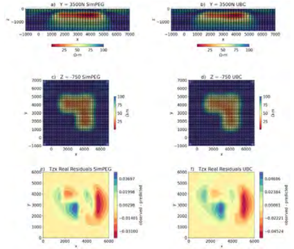
Figure 5. Recovered models obtained by inverting the synthetic ZTEM data using (a, c) SimPEG, and (b, d) the UBC E3DMT Fortran code. Panels (e), (f) show the data residual for the real part of Tzx for the SimPEG and UBC models, respectively.
