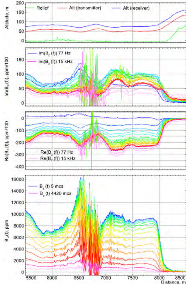
Figure 3. Industrial noise distortion on AEM data. Upper chart – the geometry of the system; central charts – imaginary and in-phase components of frequency domain data; bottom chart – time-domain data.
