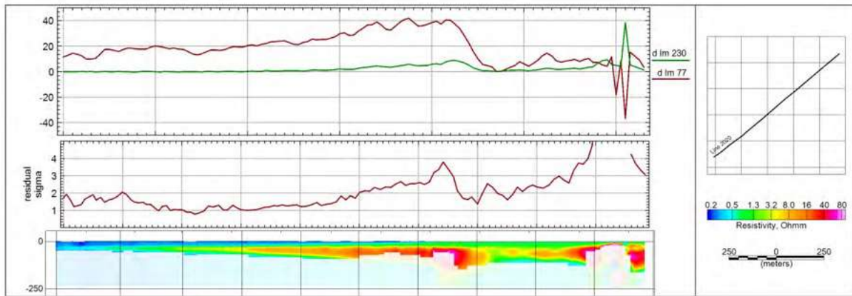
Figure 3. Inversion result in frequency domain without 77 and 230 Hz. Upper chart: d Im 77 – residual for 77 Hz, d Im 230 – residual for 230 Hz, both in ppm*100. Central chart: solution residual calculated for all other frequencies, normalized by the signal RMS. Bottom: the resistivity section.
