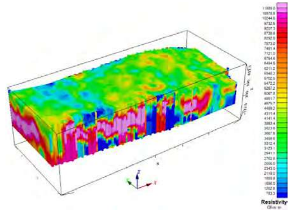
Figure 7. Electrical resistivity 3D stitched model.
