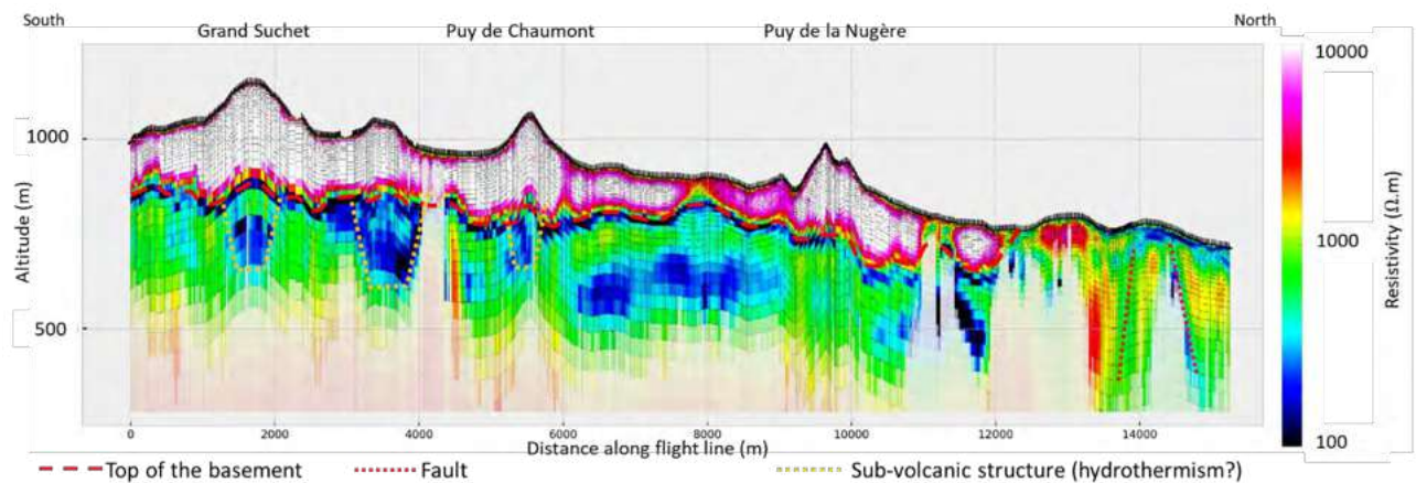
Figure 2 : South-North cross-section, located in Figure. Red dashed line highlights the contact between basement and volcanic cover. We interpret the thin low resistivity layer (dark blue) that underlies highly resistive volcanism as weathered (clay-rich) basement.
