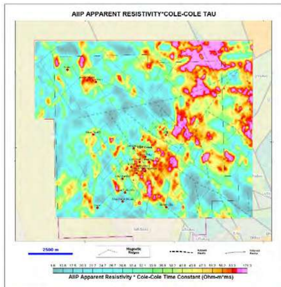
Figure 9: VTEM AIIP ResTau (Resistivity*Time Constant) Product, over mineral occurrences & known/inferred faults (dashed lines), and magnetic ridges.
