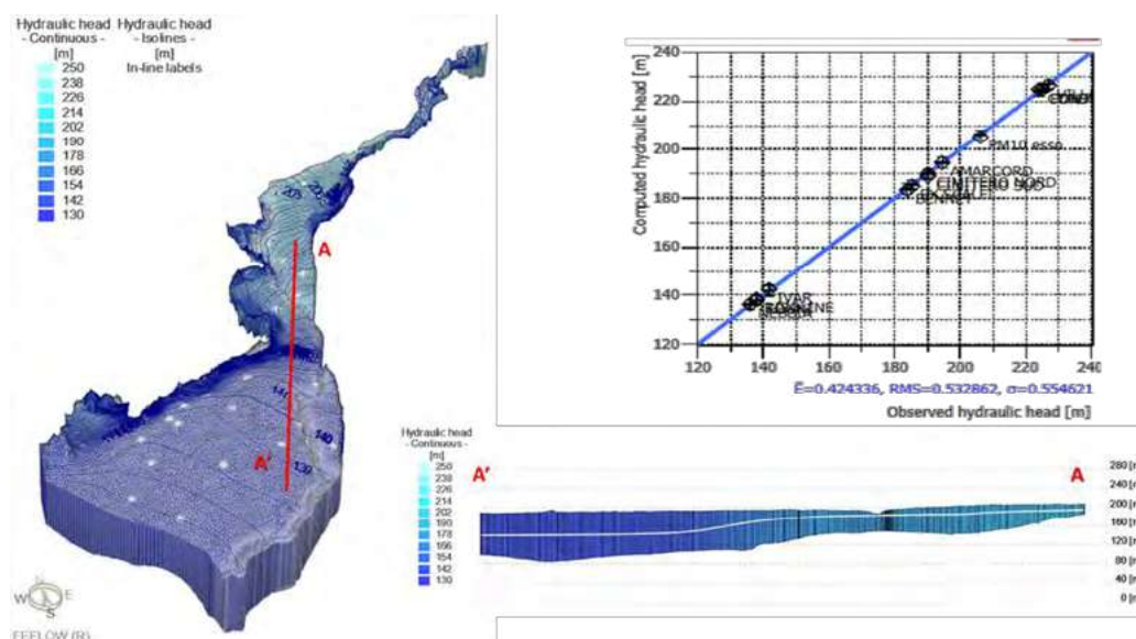
Figure 4. Results of steady-state model calibration.
