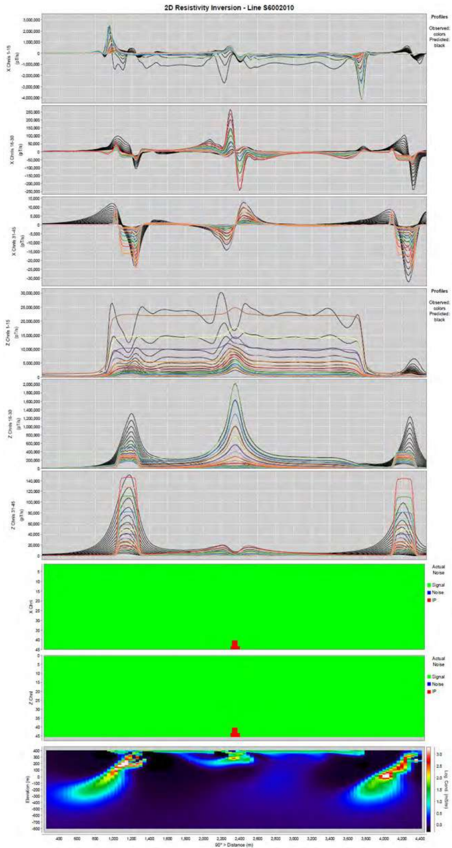
Figure 16. VTEM plus EM2.5D Inversion 6002010 with SPM (X/Z Components)
