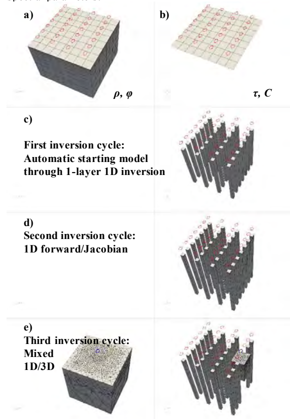
Figure 1. EEMverter multi-cycle inversion scheme for 3D AEM inversion with Induced polarization. a) Model mesh for resistivity \rho and phase \phi , with depth variability, with red polygons representing AEM frames. b) Model mesh for relaxation time \tau and frequency exponent C , without depth variability. c) First inversion cycle for computation of automatic starting model, with 1D forward meshes (grey bars) composed by only one layer. d) Second inversion cycle with 1D forward/Jacobian computations, with vertical discretization of the 1D forward meshes (grey bars). e) Third inversion cycle with mixed dimensionality of the forward/Jacobian meshes: 1D for the soundings with red frames and 3D for the soundings with blue frames (left: 3D Mesh; right: subset of the 3D mesh and 1D meshes)
