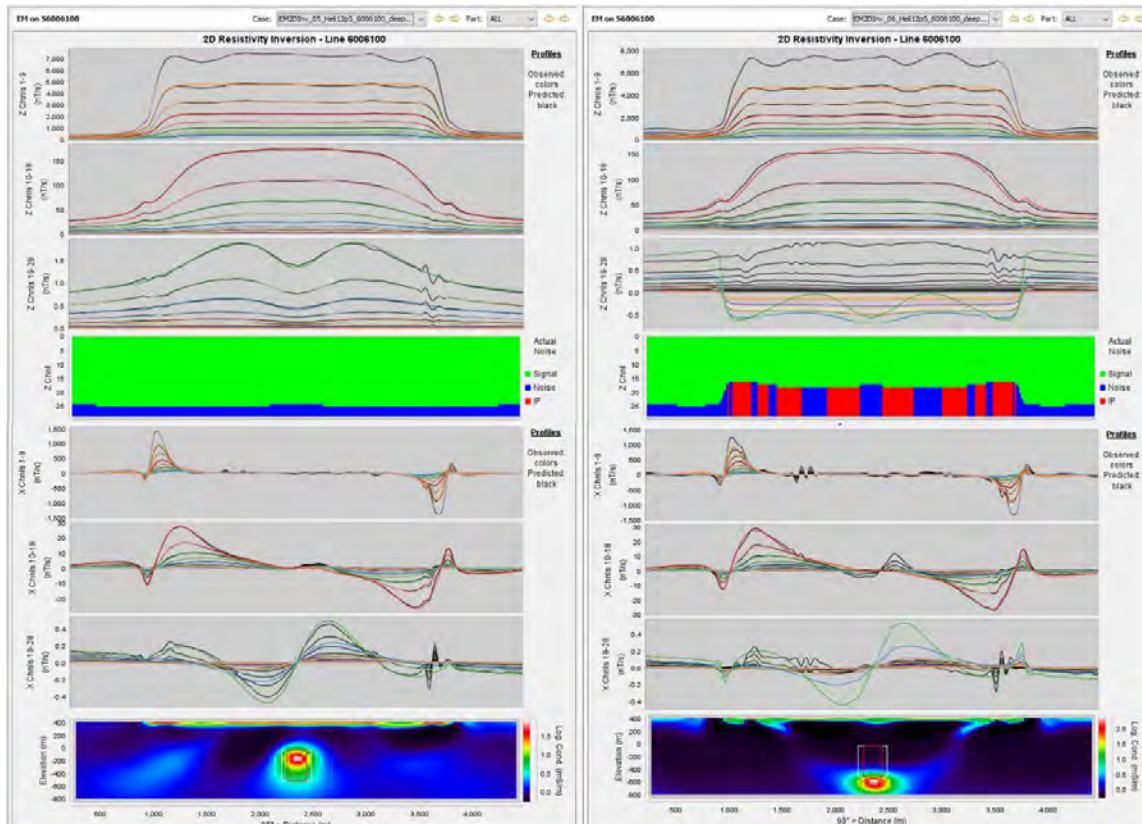
Figure 10. HeliTEM 2 12.5Hz EM2DInv 6006100 deep - without IP (left) and with IP in Cover (right)
