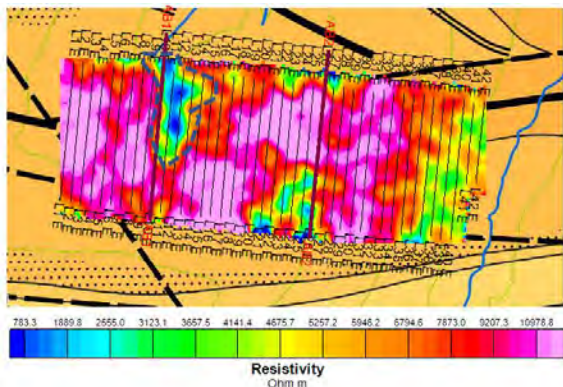
Figure 9. Electrical resistivity section with interpreted conductive anomaly (dashed line).
