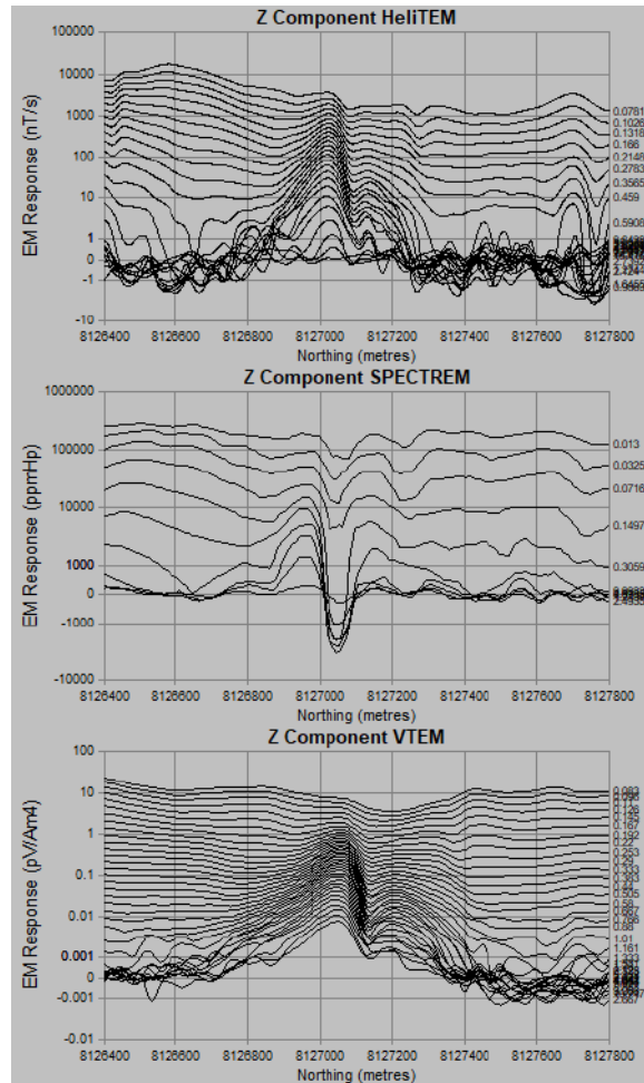
Figure 4. Coincident HeliTEM 2 and SPECTREM plus (top and centre) Z component response over target 1 and VTEM plus (bottom) Z Component response over the corresponding target
