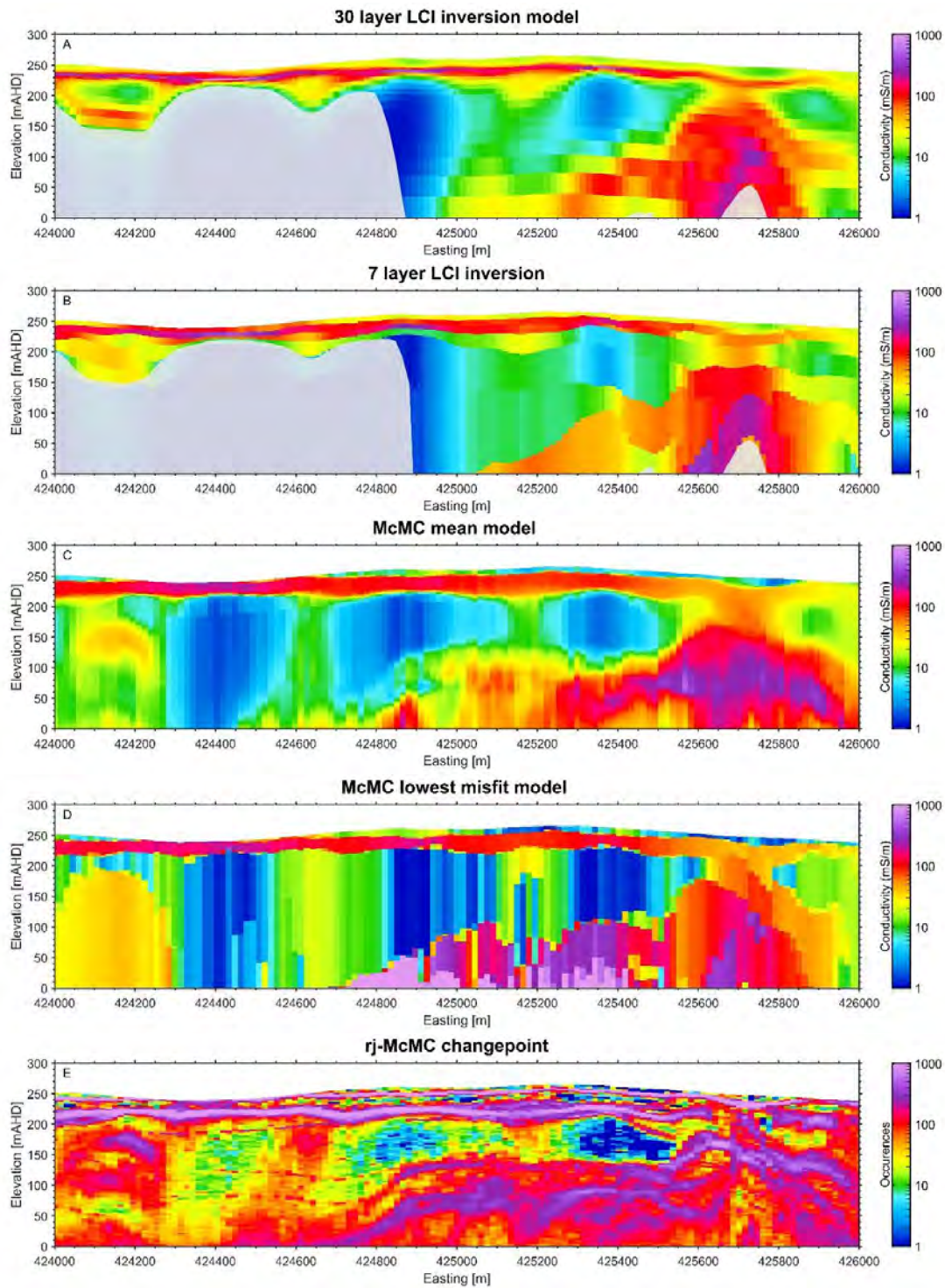
Figure 2. The results of the different inversions of line 100301 over the Gonnevillie prospect. A-B show the inversion result from using a 30 and 7 layer model discretization following a full processing of the data before inverting them using Aarhus Workbench. Panel C and D show the mean and lowest misfit models obtained by running a stochastic rj-McMC inversion.
