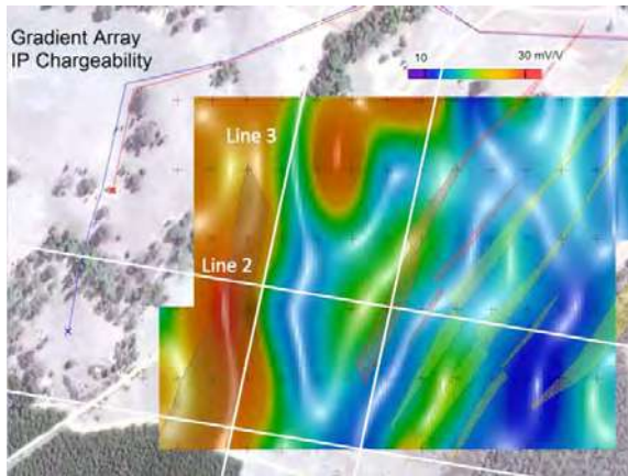
Figure 7: Gradient Array IP (Collins et al., 2022) with location of BITTEM flightlines 2 and 3.
