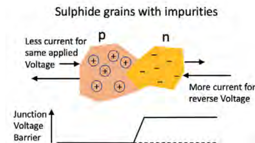
Figure 2: Semiconductor conductivity physics
