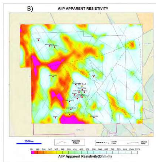
Figure 8: (A) VTEM 1D Inversion resistivity depth slice (-100m), and (B) AIIP Cole-Cole apparent resistivity, over mineral occurrences & known/inferred faults (dashed lines), and magnetic ridges.
