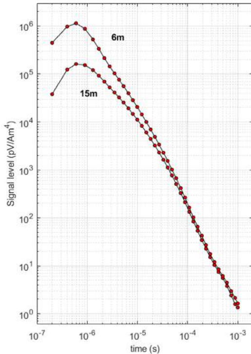
Figure 6. Transient decay curves recorded at Øbakker in 2023 for two different frame heights at approximately the same location. The data shown have been subjected to standard data processing procedures including constant bias level subtraction.
