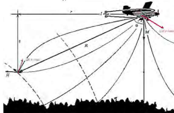
Figure 1. Airborne electromagnetic system EM4H. R - transmitter-receiver radius vector; M - vector of the magnetic moment of the exciting dipole; \Delta M - vector of the magnetic moment of the eddy current field; H - magnetic field vector of the exciting dipole; \Delta H - eddy current field vector.
