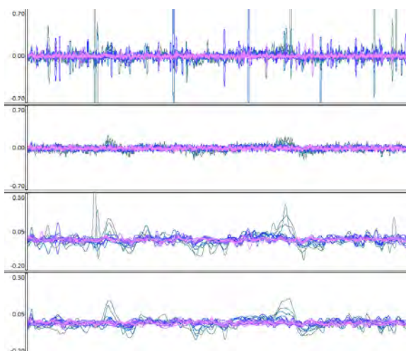
Figure 4. The same combinations of data as in Figure 3, presented over a horizontal distance of 3000m, illustrating the effective removal of noise while preserving small anomalies.
